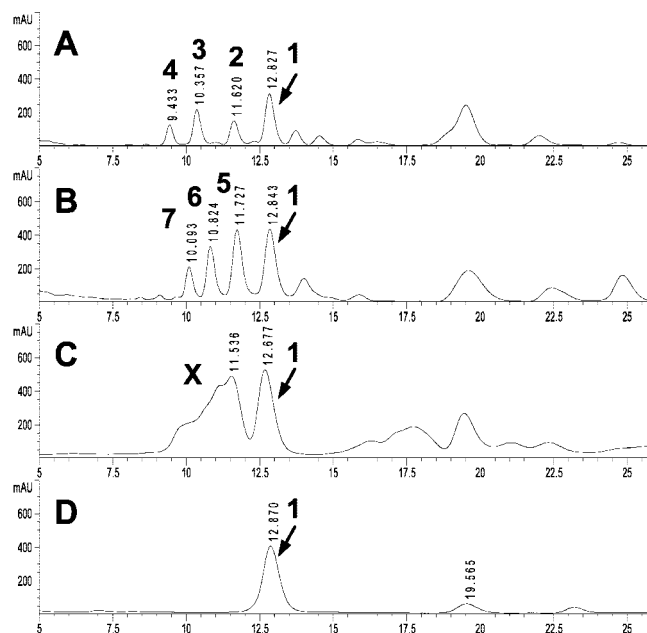
Figure 2. HPLC chromatograms of crude extracts from mycelia of B. bassiana ATCC 7159 after feeding during the fermentations with (A) DL-2-hydroxybutyric acid (Hbu), (B) DL-3-fluorophenylalanine, (C) DL-2-fluorophenylalanine, and (D) no precursor analogues. 1 , Beauvericin; 2 , beauvericin G 1 ; 3 , beauvericin G 2 ; 4 , beauvericin G 3 ; 5 , beauvericin H 1 ; 6 , beauvericin H 2 ; 7 , beauvericin H 3 ; X, unseparated mixture of putative beauvericins with one, two, and three N -methyl-L-2-fluorophenylalanine(s) instead of N -methyl-L-Phe.
